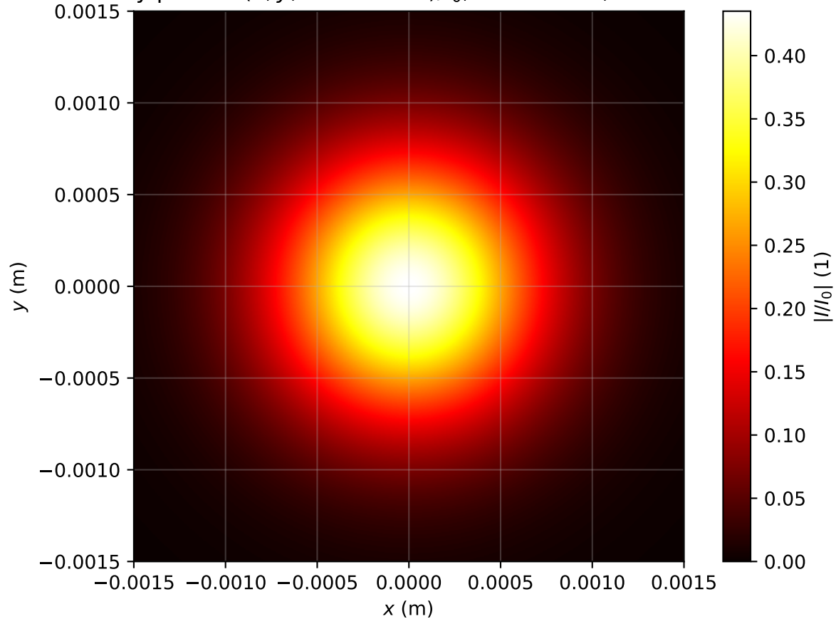
Intensity profile I(x, y, z = 3.264m)/I_0 , P_{in}=0.4P_{cr} , artificial time
